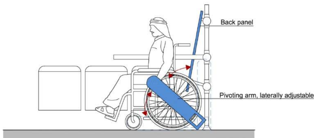
Figure 117. Rear-facing securement with pivoting aisle arm - securement technology for low transportation in buses and rail
