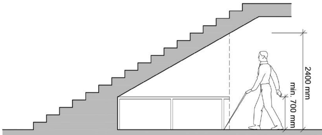
Figure 23. Spaces under stairs shall be protected
