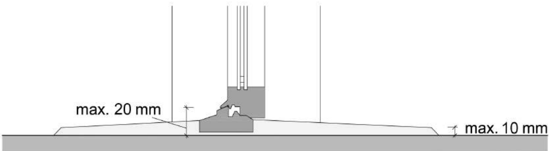
Figure 100. Maximum threshold rise
