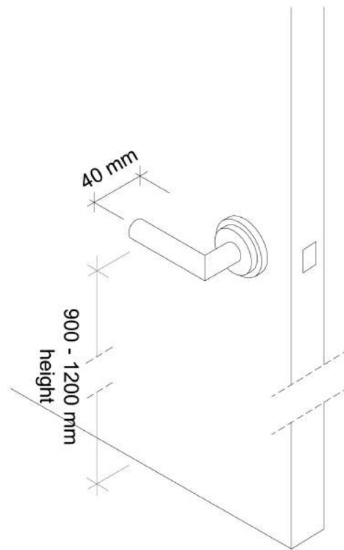
Figure 30. Door handle
