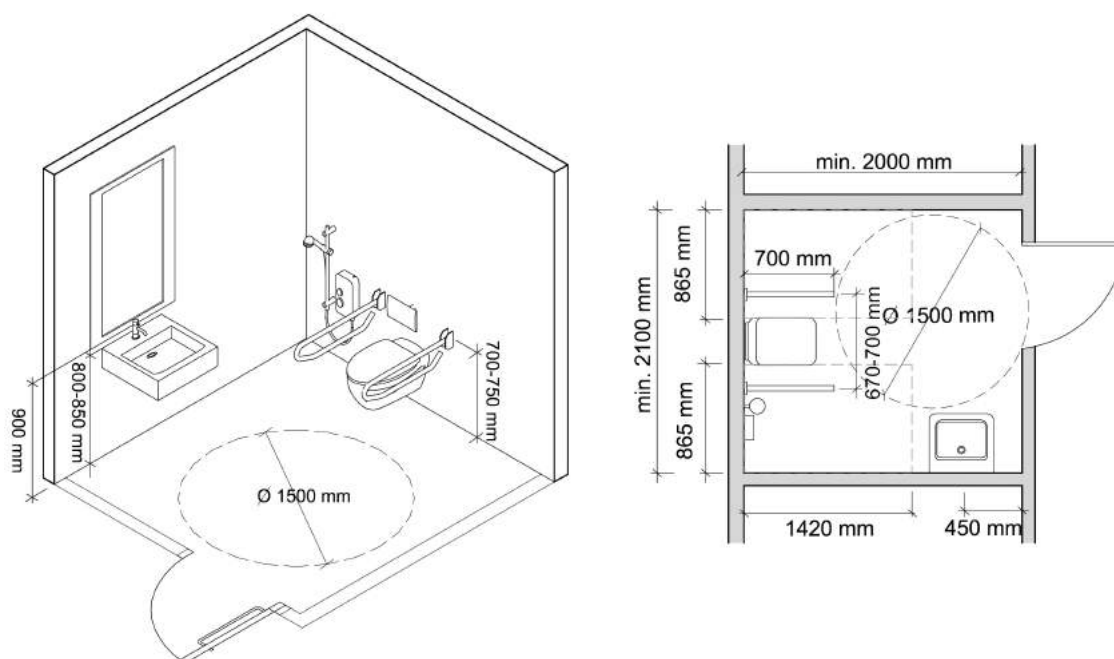
Figure 43. Transfer area on both sides of the toilet
