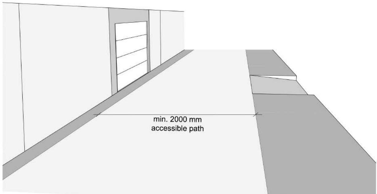
Figure 73. Possible solution to provide access to garages
