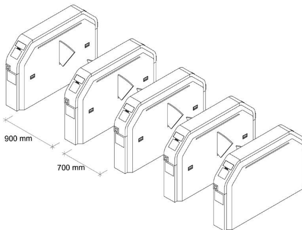
Figure 95. Access control barrier with at least one accessible gate
