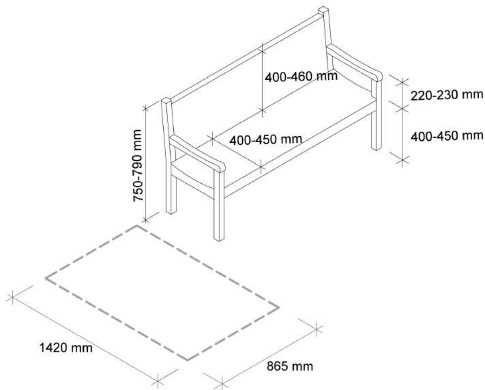
Figure 55. Bench with lateral interaction area
